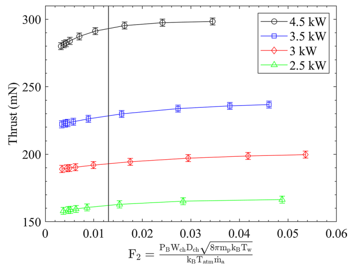
Fig. 2 Thrust versus F_2 = \frac{P_B W_{ch} D_{ch} \sqrt{8\pi m_p k_B T_w}}{k_B T_{atm} \dot{m}_a} at different anode flow rates at constant discharge voltage, corresponding to four different discharge powers. The vertical line is at the selected value of F_2^0 = 0.013 . Data adapted from Ref. [1]
