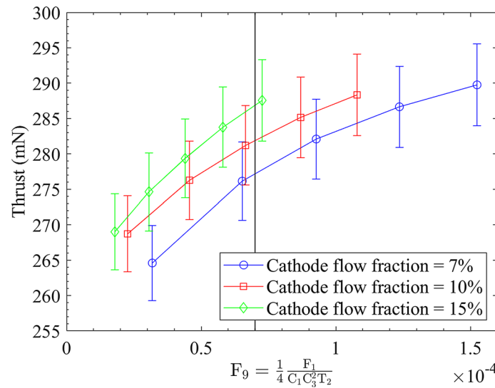
Fig. 7 Thrust versus F_9 = \frac{1}{4} \frac{F_1}{C_1 C_3^2 T_2} at different cathode flow fractions. The vertical line is at the selected value of F_9^0 = 7 \times 10^{-5} . Data adapted from Ref. [3]
