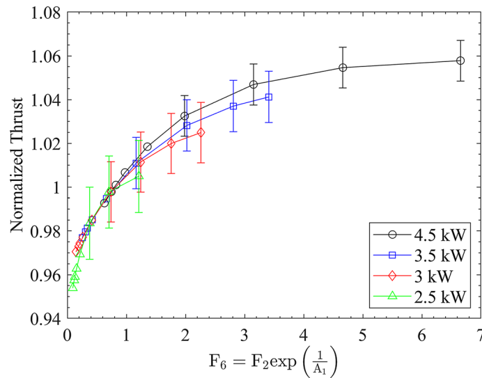
Fig. 11 Normalized thrust versus F_6 = F_2 \exp\left(\frac{1}{A_1}\right) evaluated at F_6^0 = 0.8 for different anode flow rates at constant discharge voltage, corresponding to four different discharge powers. Background pressures vary from 1 to 14 \mu\text{Torr-Xe} . For readability, certain error bars are omitted. Data adapted from Ref. [1]
