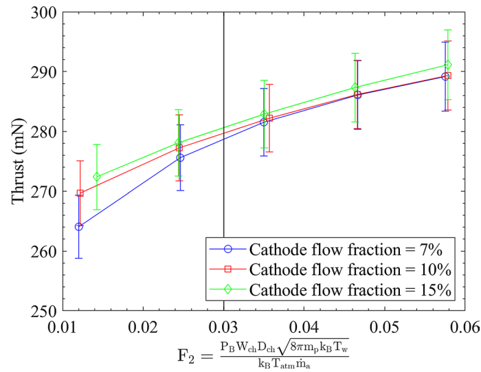
Fig. 6 Thrust versus F_2 = \frac{P_B W_{ch} D_{ch} \sqrt{8\pi m_p k_B T_w}}{k_B T_{atm} \dot{m}_a} at different cathode flow fractions. The vertical line is at the selected value of F_2^0 = 0.03 . Data adapted from Ref. [3]
