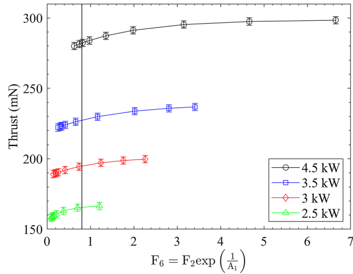
Fig. 3 Thrust versus F_6 = F_2 \exp\left(\frac{1}{A_1}\right) at different anode flow rates at constant discharge voltage, corresponding to four different discharge powers. The vertical line is at the selected value of F_6^0 = 0.8 . Data adapted from Ref. [1]
