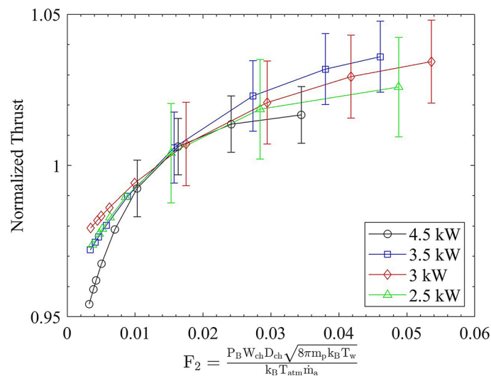
Fig. 10 Normalized thrust versus F_2 = \frac{P_B W_{ch} D_{ch} \sqrt{8 \pi m_p k_B T_w}}{k_B T_{attm} \dot{m}_a} evaluated at F_2^0 = 0.013 for different anode flow rates at constant discharge voltage, corresponding to four different discharge powers. Background pressures vary from 1 to 14 \mu\text{Torr-Xe} . For readability, certain error bars are omitted. Data adapted from Ref. [1]
