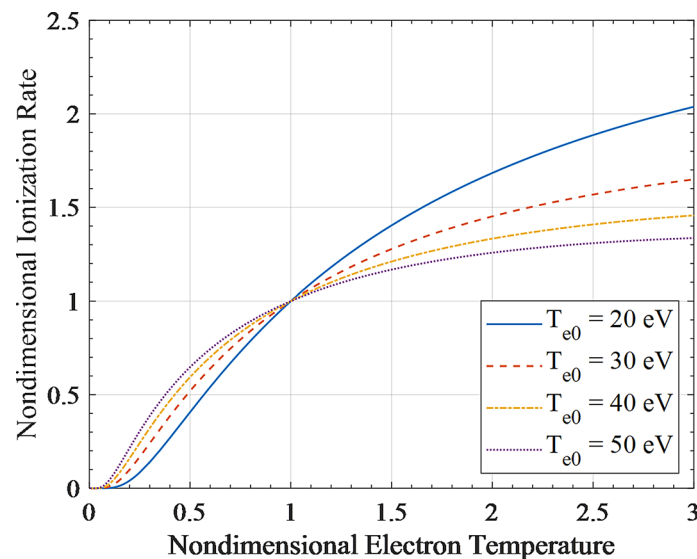
Fig. 8 Nondimensional ionization rate of xenon atom, k_{iz1}^* , as a function of nondimensional electron temperature, T_e^* for various T_{e0}
