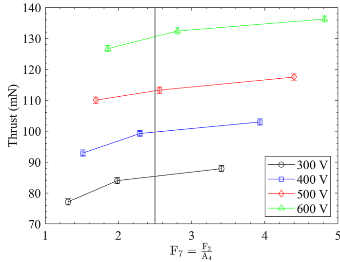
Fig. 5 Thrust versus F_7 = \frac{F_2}{A_4} at different discharge voltages at constant flow rate. The vertical line is at the selected value of F_7^0 = 2.5 . Data adapted from Ref. [2]
