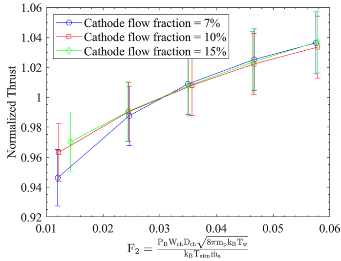
Fig. 14 Normalized thrust as a function of F_2 = \frac{P_B W_{ch} D_{ch} \sqrt{8\pi m_p k_B T_w}}{k_B T_{atm} \dot{m}_a} evaluated at F_2^0 = 0.03 for different cathode flow fractions. Background pressures vary from 5 to 20 \mu Torr-Xe. Data adapted from Ref. [3]
