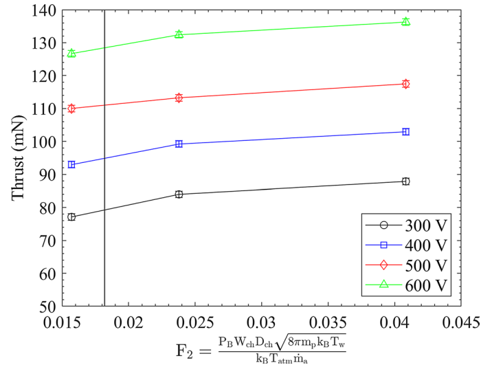
Fig. 4 Thrust versus F_2 = \frac{P_B W_{ch} D_{ch} \sqrt{8\pi m_p k_B T_w}}{k_B T_{atm} \dot{m}_a} at different discharge voltages at constant flow rate. The vertical line is at the selected value of F_2^0 = 0.0182 . Data adapted from Ref. [2]
