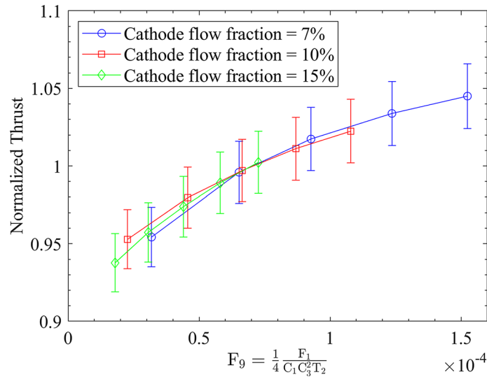
Fig. 15 Normalized thrust as a function of F_9 = \frac{1}{4} \frac{F_1}{C_1 C_3^2 T_2} evaluated at F_9^0 = 7 \times 10^{-5} for different cathode flow fractions. Background pressures vary from 5 to 20 \mu Torr-Xe. Data adapted from Ref. [3]
