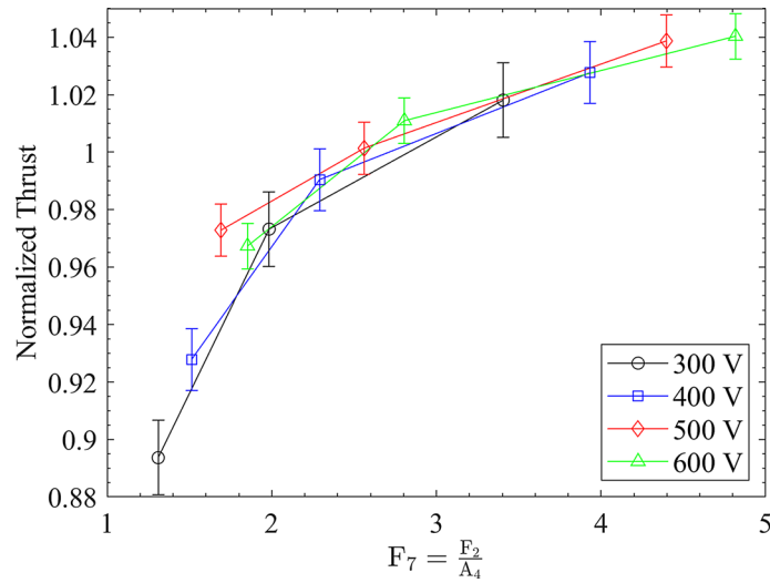
Fig. 12 Normalized thrust as a function of F_7 = \frac{F_2}{A_4} evaluated at F_7^0 = 2.5 for different discharge voltages at constant flow rate. Background pressures vary from 5 to 14 \mu\text{Torr-Xe} . Data adapted from Ref. [2]
