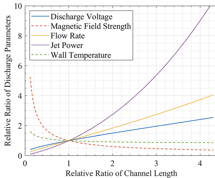
Fig. 9 Relative ratio in discharge parameters required for constant A_1 , A_2 , A_3 , T_1 , and T_2 as a function of channel length. Reference condition is xenon at 300V, \frac{\dot{m}_a}{\pi W_{ch} D_{ch}} = 10^{-3} \frac{\text{kg}}{\text{s} \cdot \text{m}^2} , L_{ch} = 30 \text{ mm} , W_{ch} = 30 \text{ mm} , D_{ch} = 100 , and \sigma_{SEE} = 0.5
