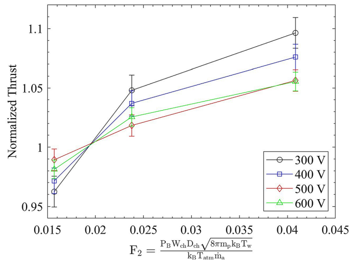
Fig. 13 Normalized thrust as a function of F_2 = \frac{P_B W_{ch} D_{ch} \sqrt{8\pi m_p k_B T_w}}{k_B T_{atm} \dot{m}_a} evaluated at F_2^0 = 0.0182 for different discharge voltages at constant flow rate. Background pressures vary from 5 to 14 \mu\text{Torr-Xe} . Data adapted from Ref. [2]
