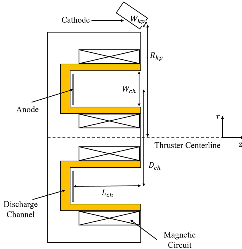
Fig. 1 Schematic of an annular HET. Geometric parameters L_{ch} , W_{ch} , D_{ch} , W_{kp} , and R_{kp} are shown
